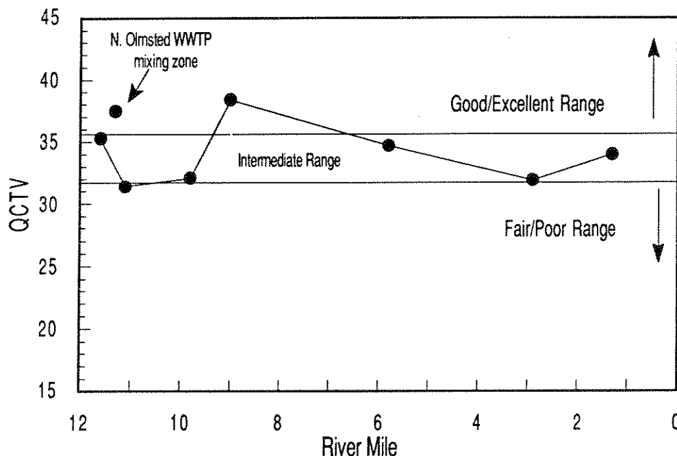
Figure 7. Longitudinal trend of Qualitative Community Tolerance Values (QCTV) in the Rocky River, 1992.
