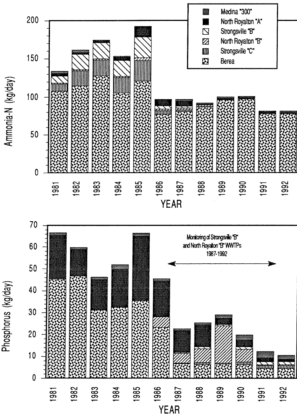
Figure 38. Cumulative 50th percentile annual ammonia-N and phosphorus loadings from six dischargers to the East Branch Rocky River study area, 1981-1992.
