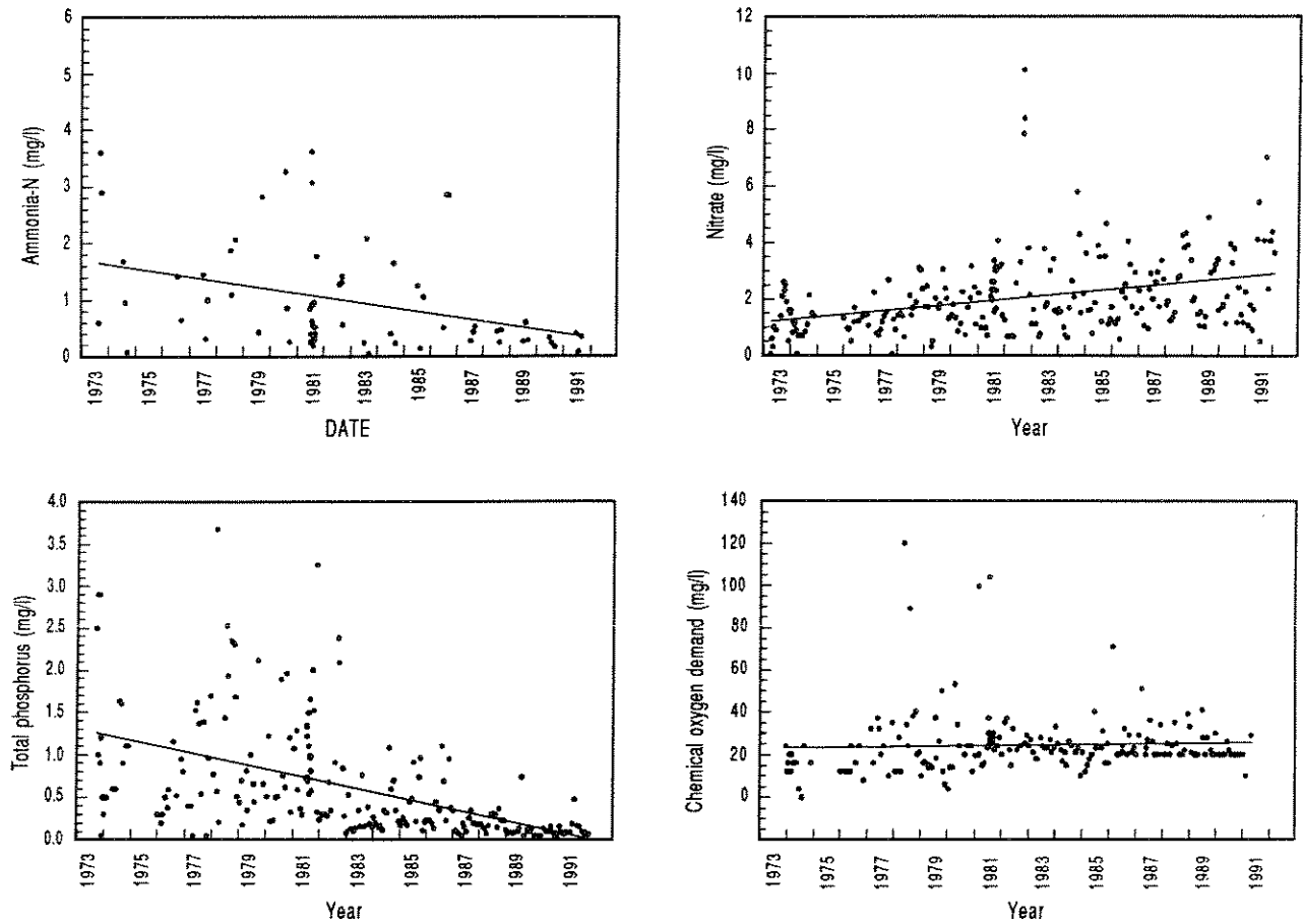
Figure 28. Linear regressions of nitrate ( p < 0.001 ), phosphorus ( p < 0.001 ), chemical oxygen demand ( p < 0.20 ) and 3rd quarter ammonia-N ( p < 0.01 ) concentrations from grab samples collected from the Rocky River at Cedar Point Rd. (RM 12.7), 1973-1992.
