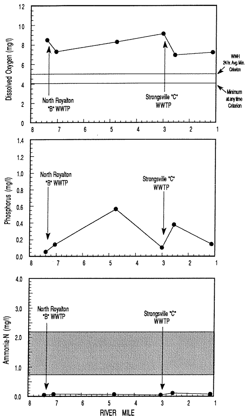
Figure 23. Longitudinal trend of mean D.O., phosphorus and ammonia-N in Baldwin Creek, 1992. Shaded area represents the range of ammonia WQS criteria between the 90th and 25th percentile pH and temperatures.
