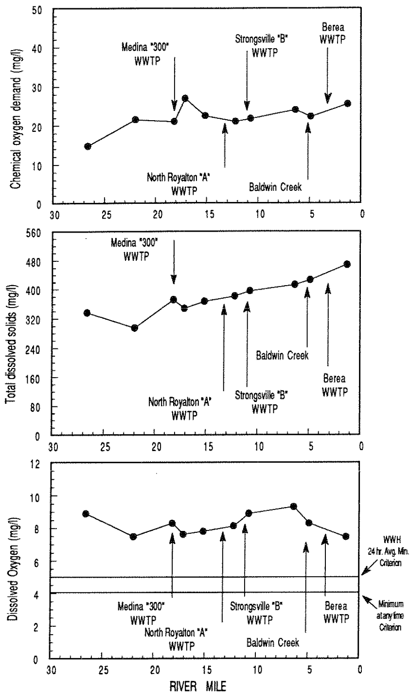
Figure 14. Longitudinal trends of mean chemical oxygen demand, total dissolved solids and dissolved oxygen from the East Branch Rocky River, 1992.
