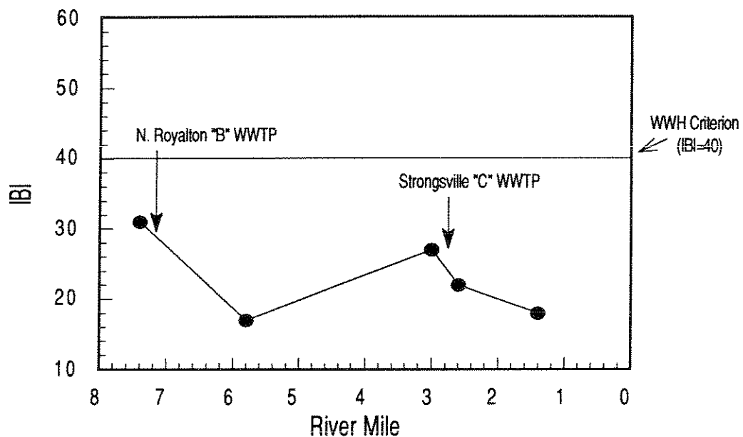
Figure 25. Longitudinal trend of the Index of Biotic Integrity (IBI) in Baldwin Creek, 1992.
