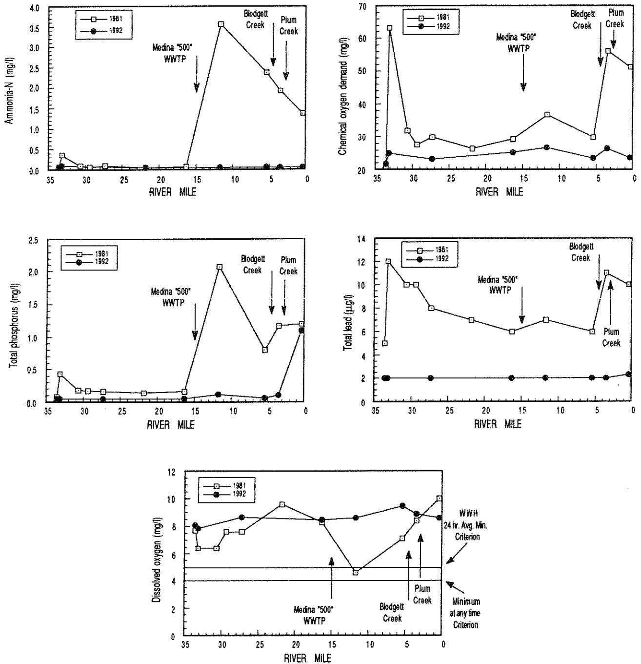
Figure 40. Longitudinal trend of mean ammonia-N, chemical oxygen demand, phosphorus, lead, and dissolved oxygen in the West Branch Rocky River study area, 1981-1992.
