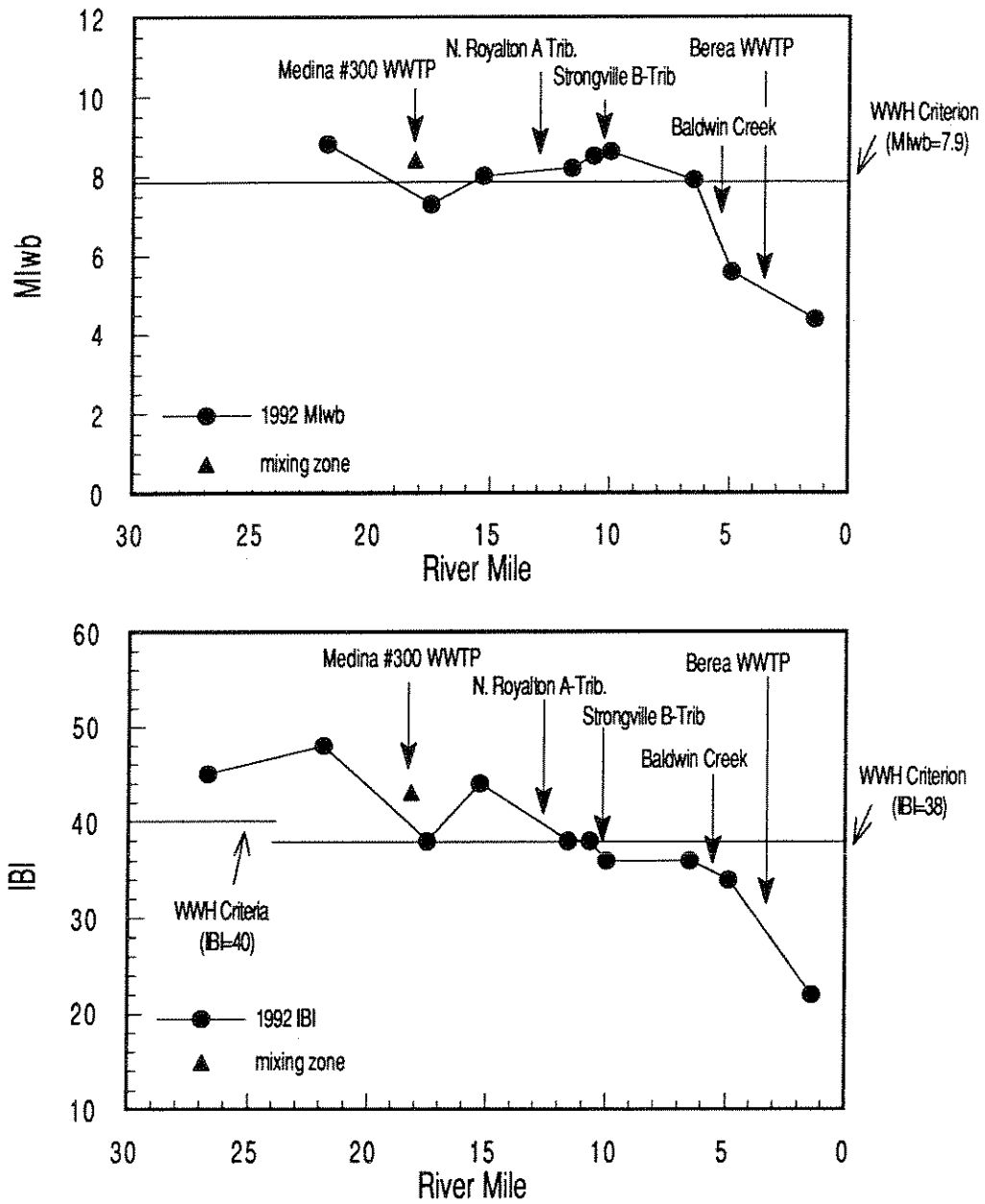
Figure 16. Longitudinal trend of the Modified Index of Well-Being (MIwb; upper) and the Index of Biotic Integrity (IBI; lower) in the East Branch Rocky River, 1992.
