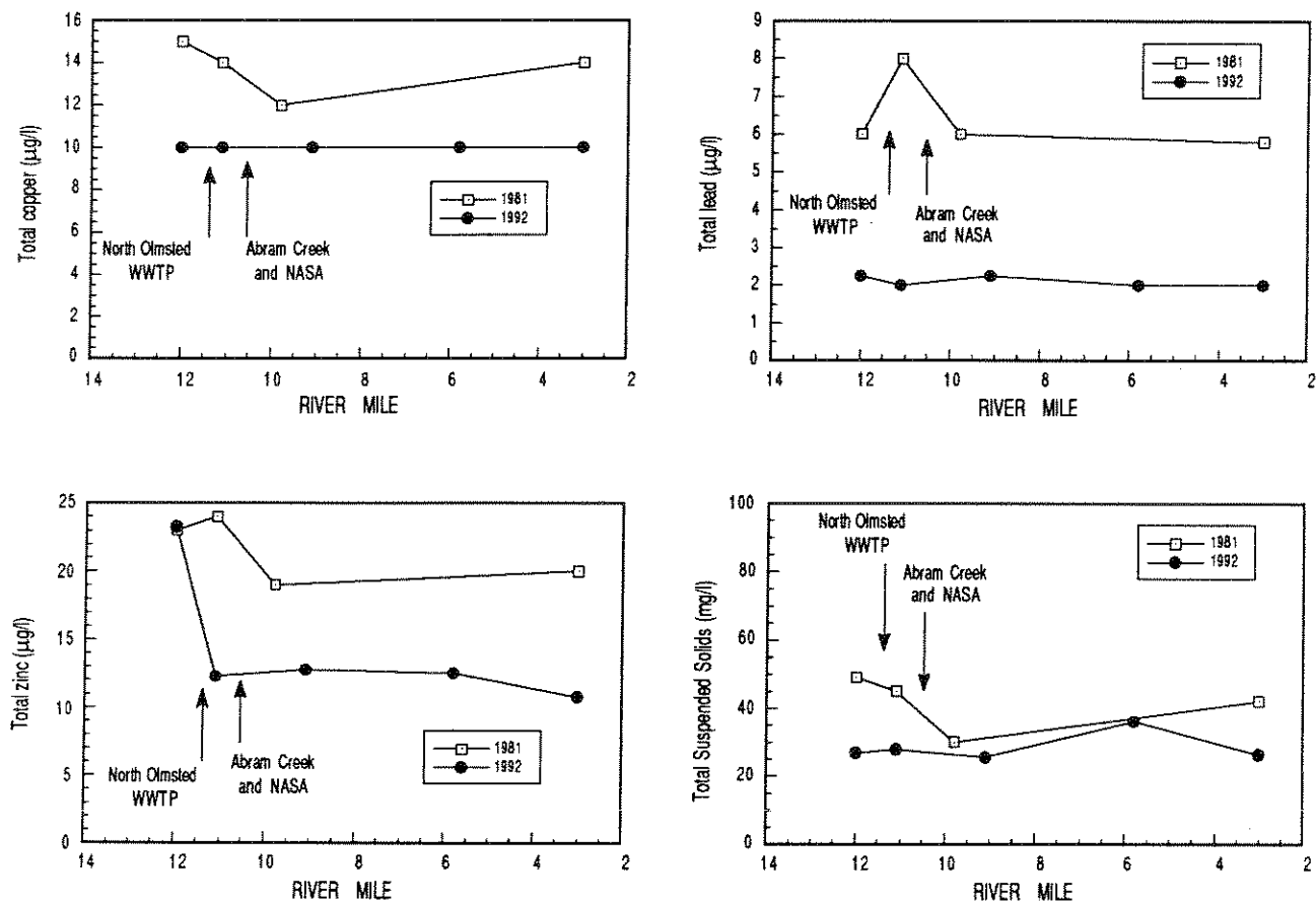
Figure 31. Longitudinal trends of mean copper, lead, zinc, and total suspended solids in the Rocky River, 1981 and 1992.
