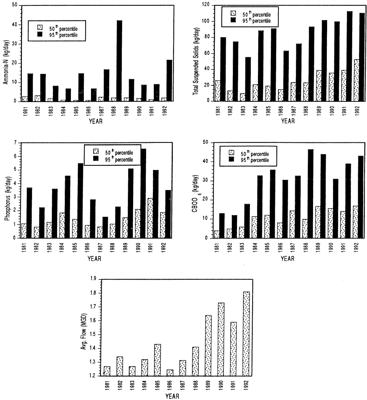
Figure 11. Average flow (MGD) and annual loadings (kg/day) of ammonia, suspended solids, phosphorus and CBOD 5 from the Medina 300 WWTP, 1981-1992. CBOD 5 loadings for 1981-1984 are calculated based on reported biochemical oxygen demand (BOD 5 ) values.
