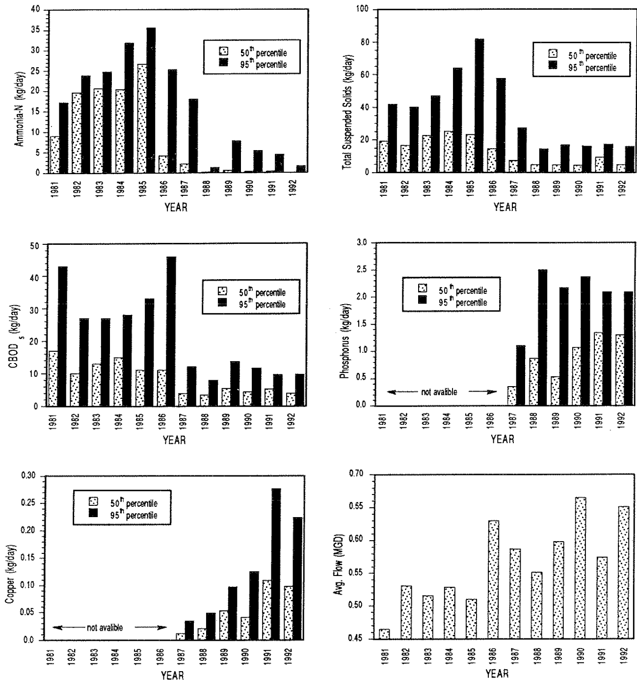
Figure 12. Average flow (MGD) and annual loadings (kg/day) of ammonia, suspended solids, CBOD 5 , phosphorus and copper from the Strongsville "B" WWTP, 1981-1992. CBOD 5 loadings for 1981-1984 are calculated based on reported biochemical oxygen demand (BOD 5 ) values.
