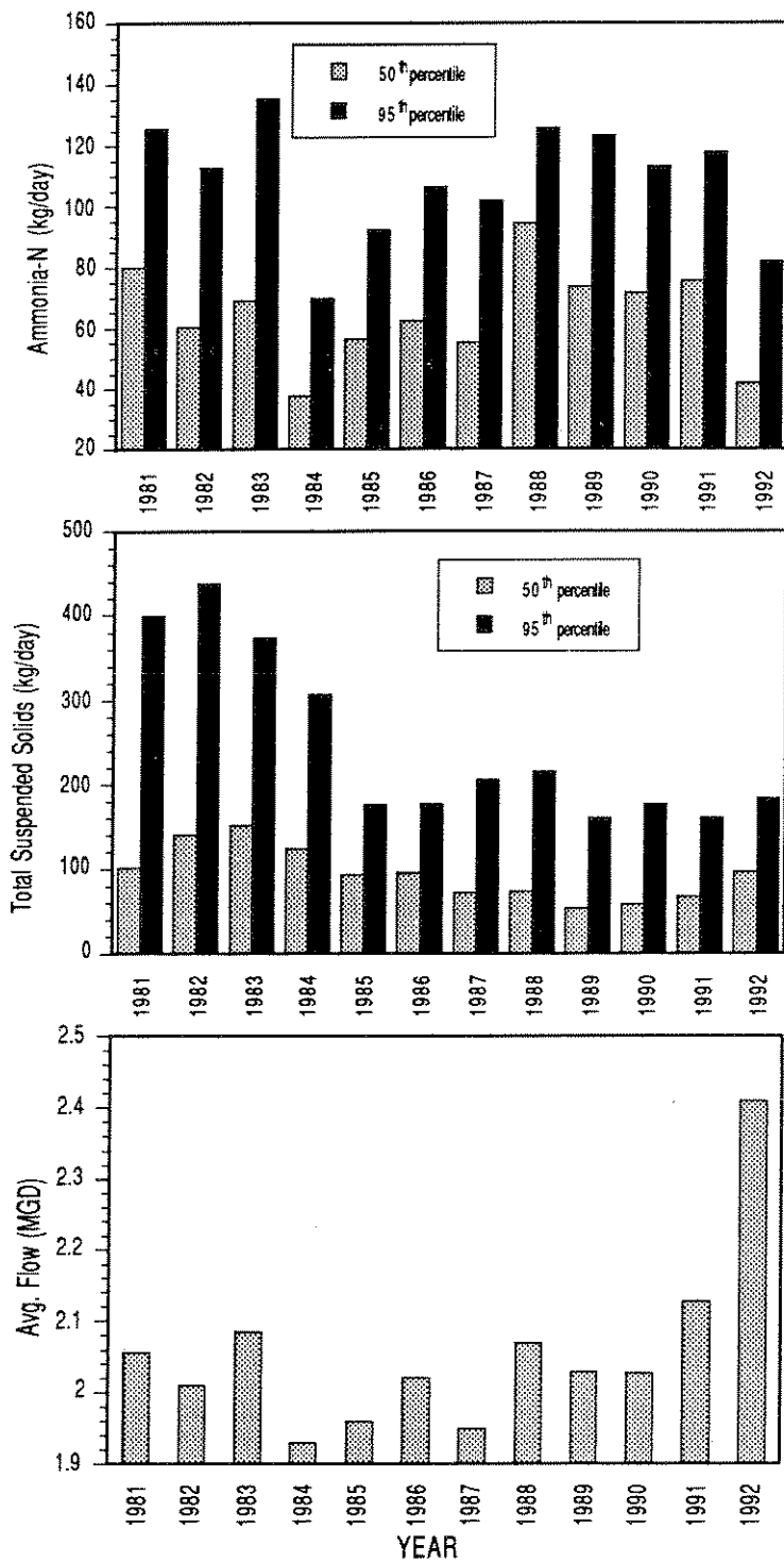
Figure 9. Average flow (MGD) and annual loadings (kg/day) of suspended solids and ammonia-N, from the Middleburg Heights WWTP, 1981-1992.
