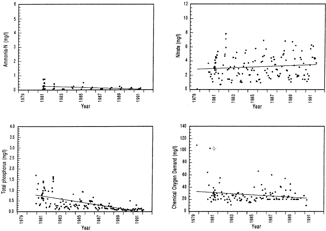
Figure 29. Linear regressions of nitrate ( p < 0.10 ), phosphorus ( p < 0.001 ), chemical oxygen demand ( p < 0.005 ) and 3rd quarter ammonia-N ( p < 0.01 ) concentrations from grab samples collected from the Rocky River at Rockcliff ford (RM 3.0), 1979-1992.
