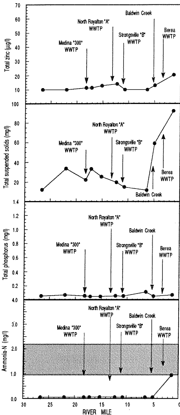
Figure 15. Longitudinal trend of mean zinc, total suspended solids, phosphorous and ammonia from the East Branch Rocky River, 1992. Shaded area represents the ammonia WQS range for 90th and 25th percentile pH and temperature values.
