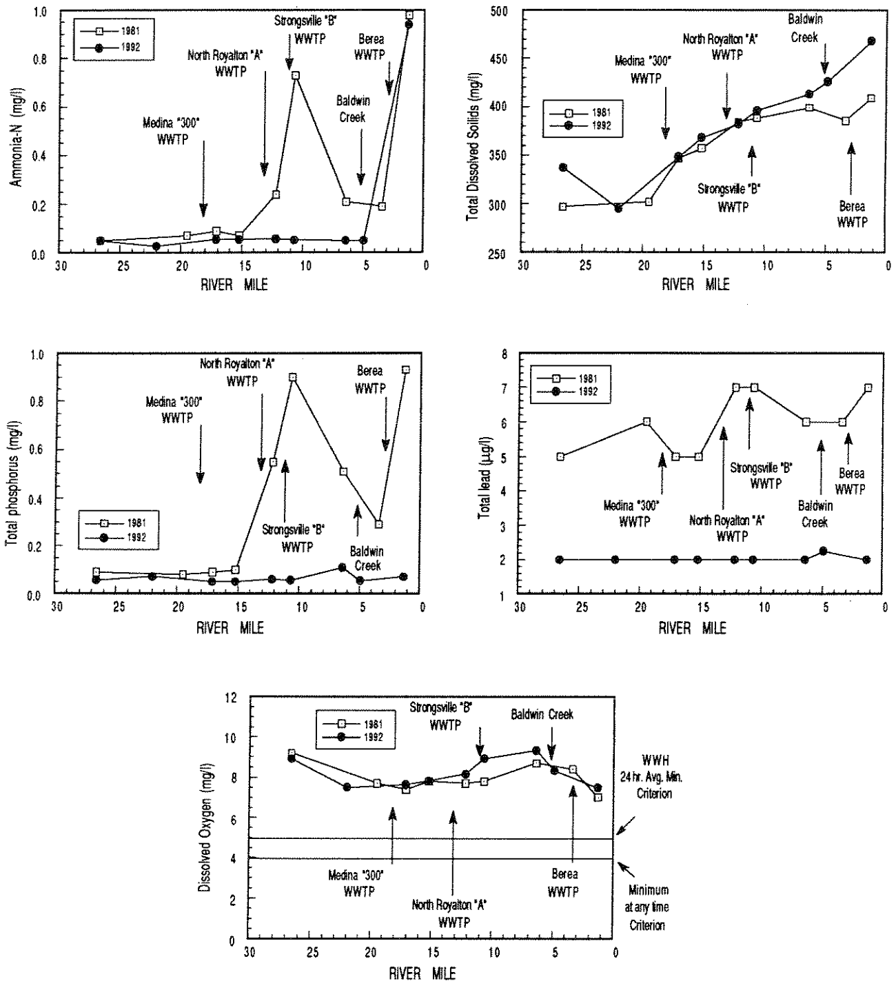
Figure 37. Longitudinal trend of mean ammonia-N, total dissolved solids, phosphorus, lead, and dissolved oxygen in the East Branch Rocky River study area, 1981-1992.
