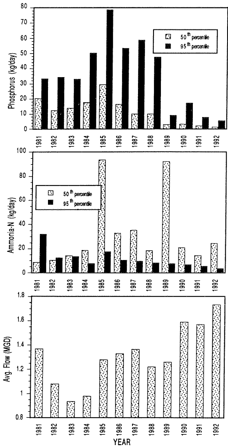
Figure 26. Average flow (MGD) and annual loadings (kg/day) of phosphorus and ammonia-N, from the North Royalton "A" WWTP to the North Royalton "A" WWTP tributary, 1981 to 1992.
