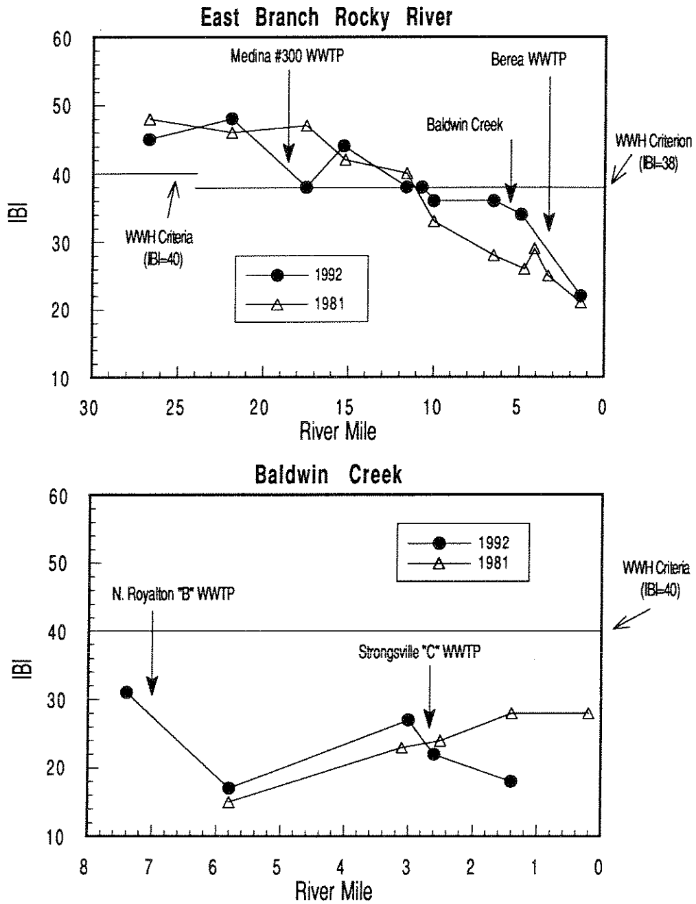
Figure 39. Longitudinal trends of the Index of Biotic Integrity (IBI) in the East Branch Rocky River and Baldwin Creek study areas, 1981 and 1992.
