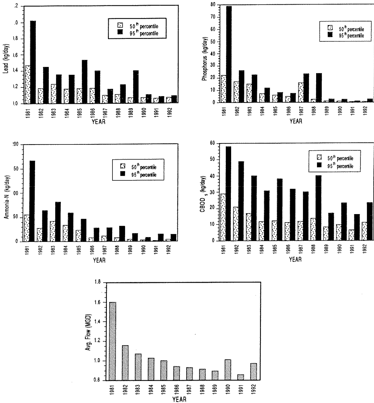
Figure 10. Average flow and annual loadings (kg/day) of lead, phosphorus, ammonia-N, and CBOD 5 from the Brookpark WWTP, 1981-1992. CBOD 5 loadings for 1981-1984 are calculated based on reported biochemical oxygen demand (BOD 5 ) values.
