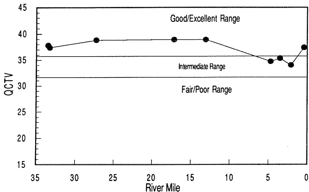
Figure 19. Longitudinal trend of the Qualitative Community Tolerance Value (QCTV) in the West Branch Rocky River, 1992.
