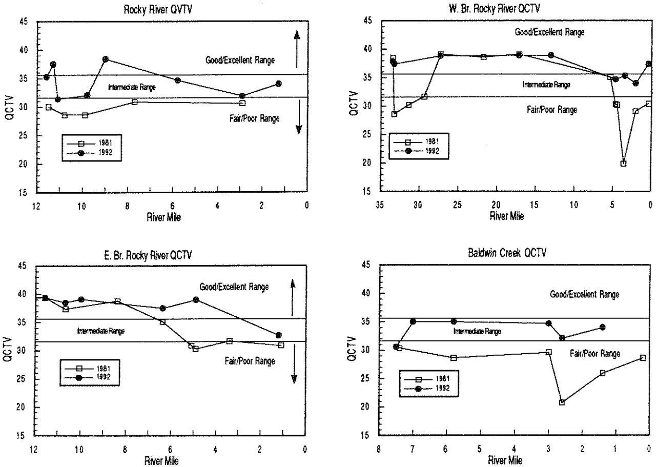
Figure 35. Longitudinal trend of Qualitative Community Tolerance Values (QCTV) scores from the Rocky River, East Branch Rocky River, West Branch Rocky River, and Baldwin Creek, 1981 and 1992.
