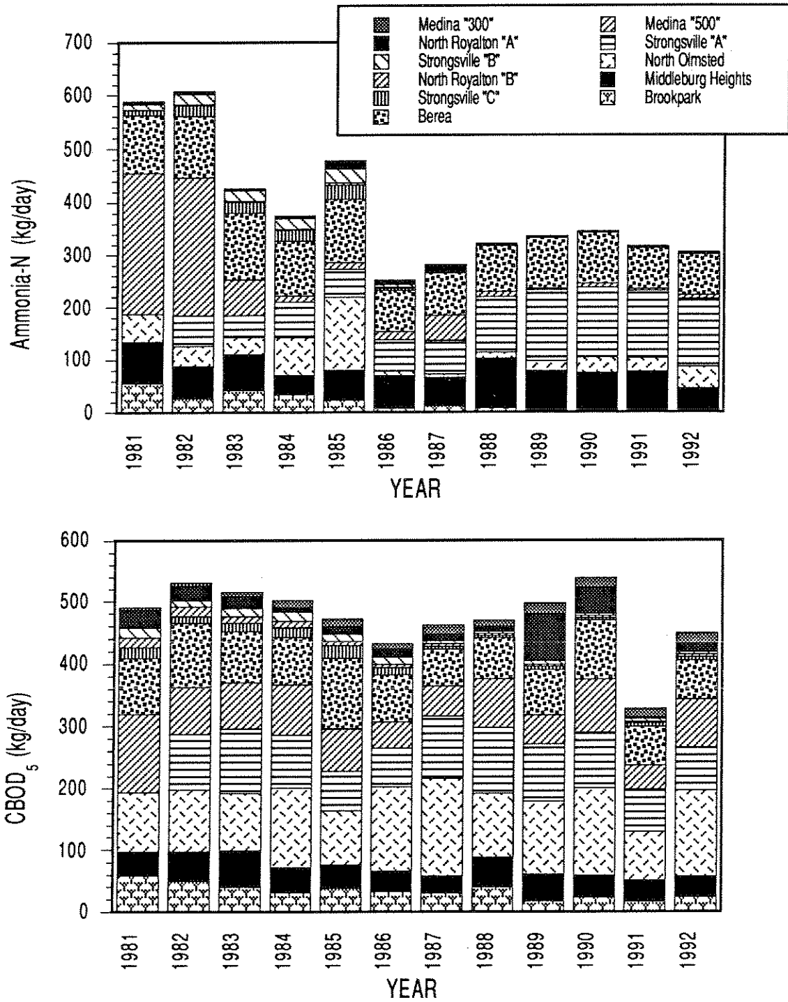
Figure 30. Cumulative 50th percentile Ammonia-N (kg/day) and CBOD 5 loadings for eleven dischargers in the Rocky River basin, 1981-1992.
