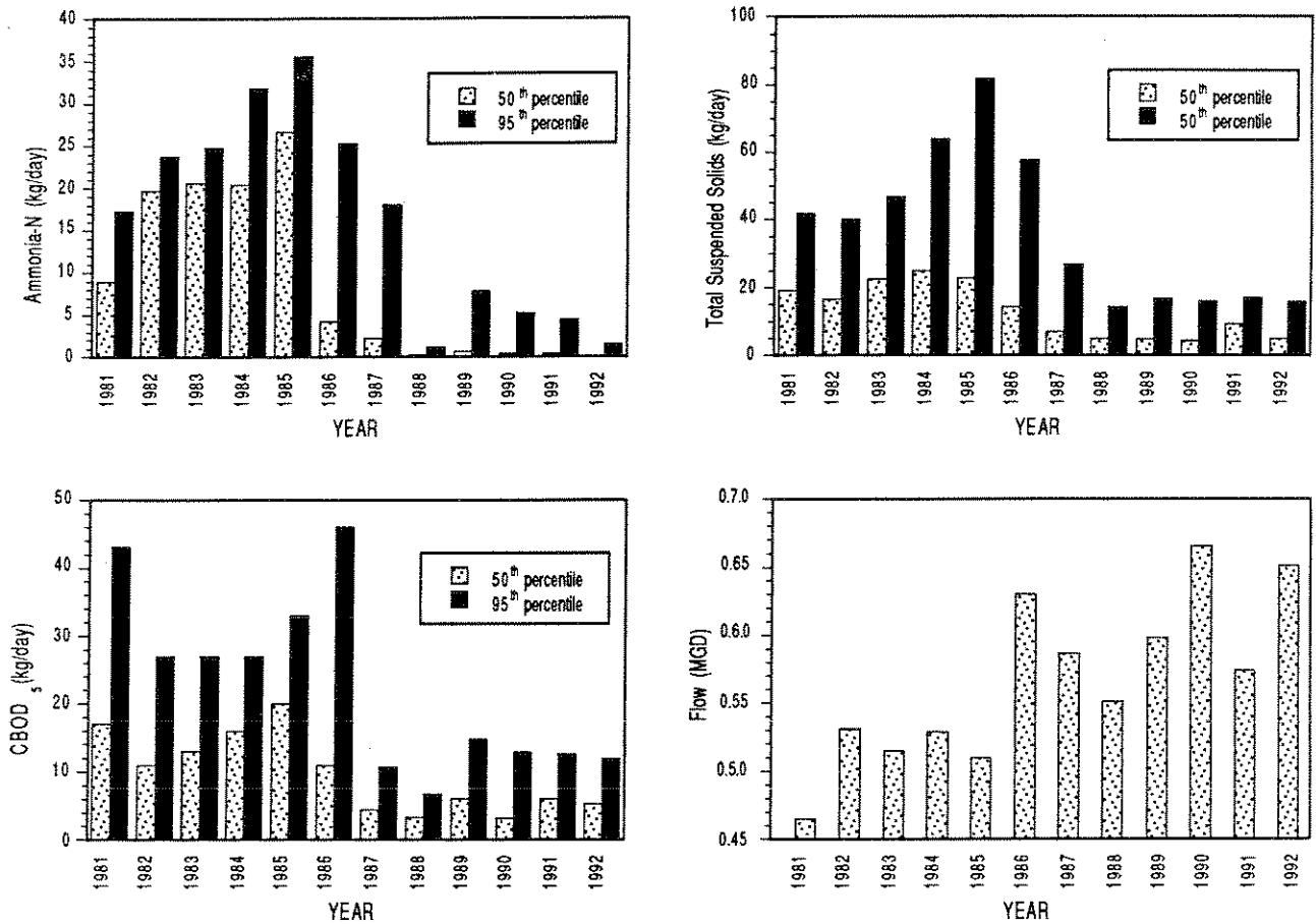
Figure 22. Average flow (MGD) and annual loadings (kg/day) of ammonia-N, total suspended solids, CBOD 5 from the Strongsville "C" WWTP to Baldwin Creek, 1981-1992. CBOD 5 loadings for 1981-1984 are calculated based on reported biochemical oxygen demand (BOD 5 ) values.
