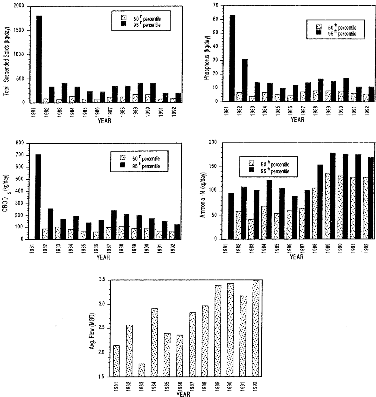
Figure 27. Average flow (MGD) and annual loadings (kg/day) of phosphorus, ammonia-N, CBOD 5 and total suspended solids from the Strongsville "A" WWTP to Blodgett Creek, 1981 to 1992. CBOD 5 loadings for 1981-1984 are calculated based on reported biochemical oxygen demand (BOD 5 ) values.
