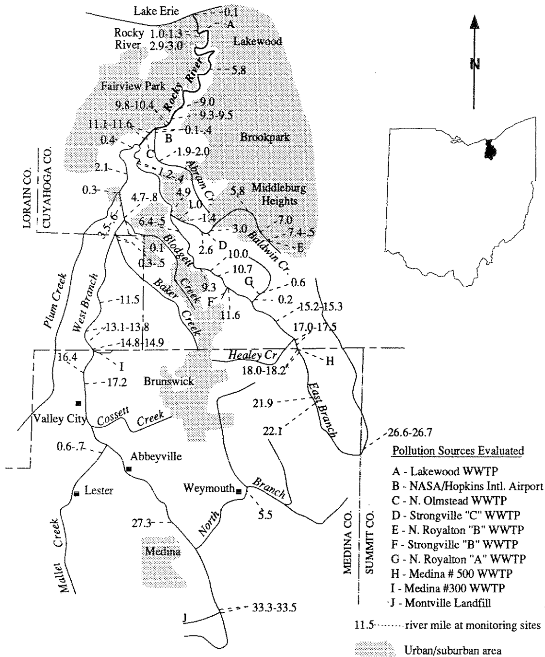
Figure 1. The Rocky River study area showing principal streams and tributaries, population centers, pollution sources, and sampling locations.
