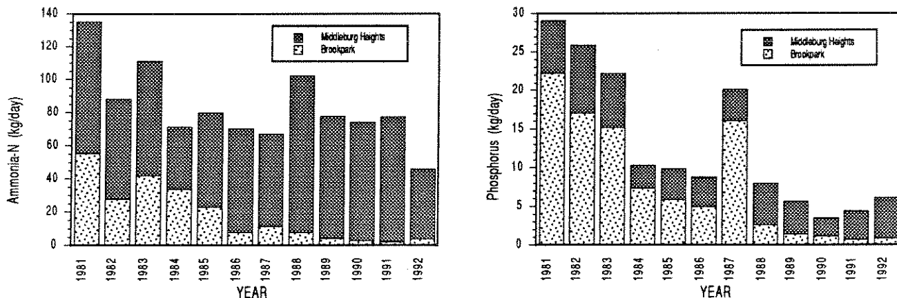
Figure 33. Cumulative 50th percentile ammonia-N and phosphorus loadings in Abram Creek, 1981-1992.
