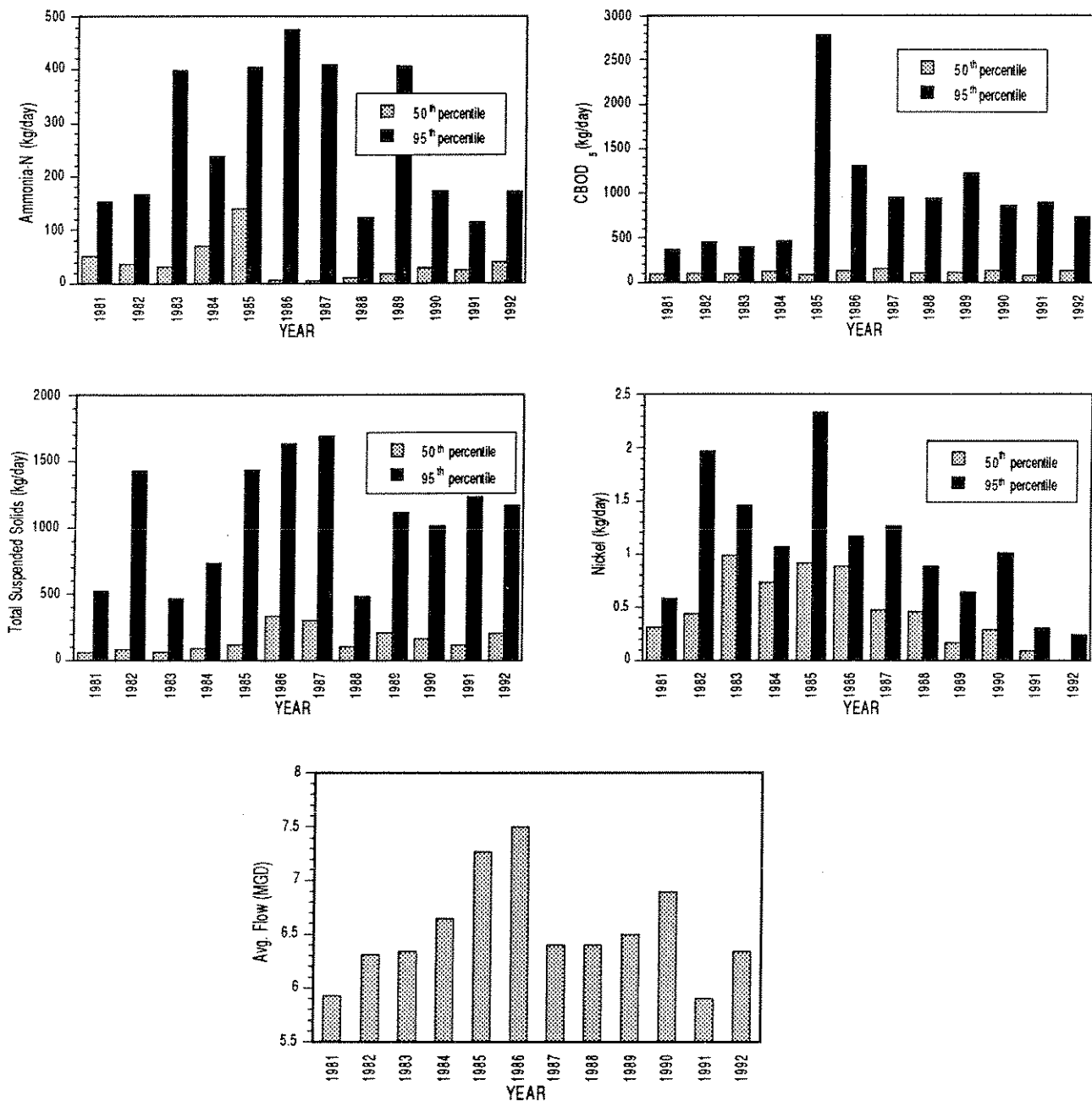
Figure 3. Annual loadings (kg/day) of ammonia-N, carbonaceous biochemical oxygen demand (CBOD 5 ), total suspended solids (TSS), nickel, and average flow from the North Olmsted WWTP to the Rocky River, 1981 to 1992. CBOD 5 loading for 1981 through 1984 are calculated based on reported five-day biochemical oxygen demand (BOD 5 ) values.
