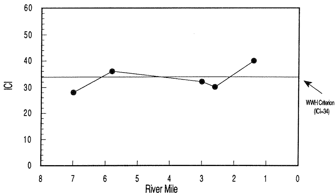
Figure 24. Longitudinal trend of the Invertebrate Community Index (ICI) in Baldwin Creek, 1992.
