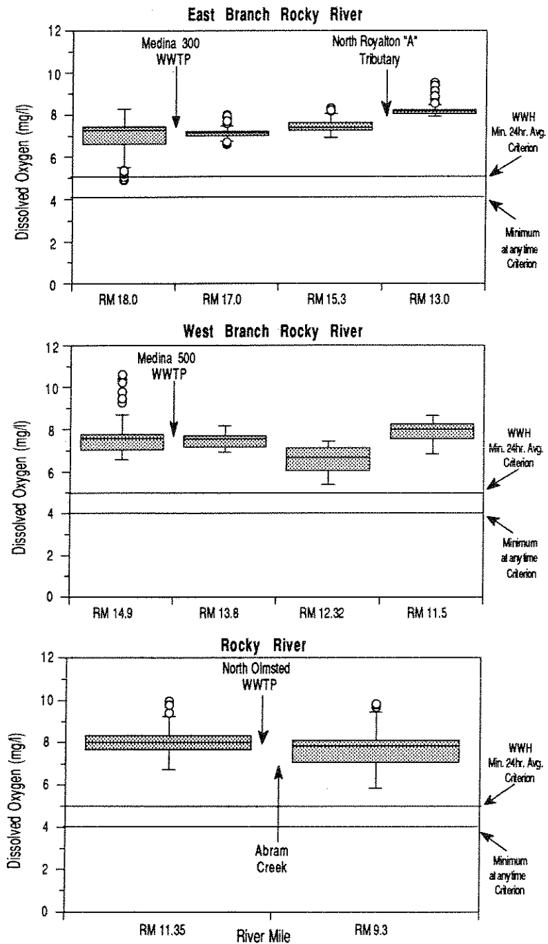
Figure 6. Boxplots of dissolved oxygen data recorded with continuous monitors at selected locations in the East Branch, West Branch, and the Rocky River mainstem, August 25-28, 1992.
