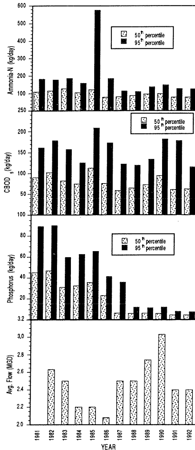
Figure 13. Average flow (MGD) and annual loadings (kg/day) of ammonia, suspended solids, CBOD 5 and phosphorus from the Berea WWTP, 1981-1992. CBOD 5 loadings for 1981-1984 are calculated based on reported biochemical oxygen demand (BOD 5 ) values.
