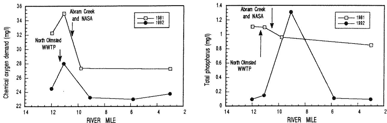
Figure 32 Longitudinal trends of mean chemical oxygen demand (COD) and phosphorus in the Rocky River, 1981 and 1992
