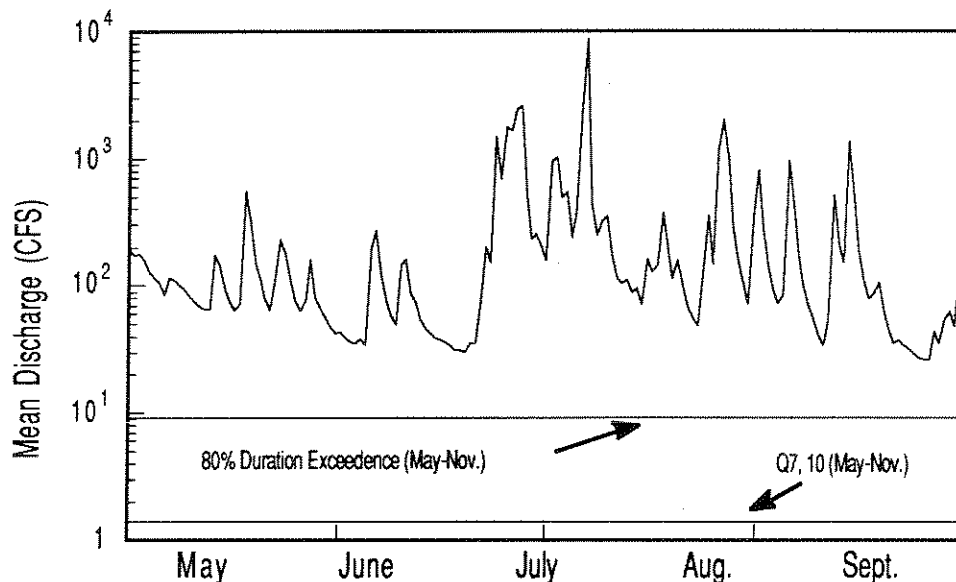
Figure 4. Flow hydrograph for the Rocky River at Cedar Point Rd. (RM 12.07), May through September, 1992 (USGS 1992). May through November low-flow conditions ( Q_{7,10} [1.4 cfs] and 80% duration flow [9.2 cfs]); period of record 1923 to 1978 (USGS 1981)
