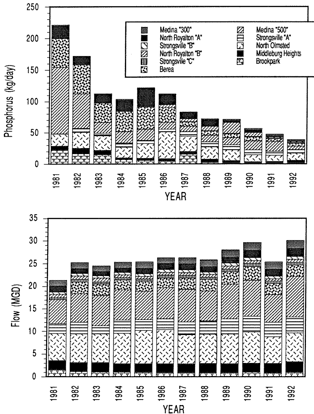
Figure 34. Cumulative 50th percentile phosphorus (kg/day) and flow (MGD) for eleven discharges in the Rocky River basin.
