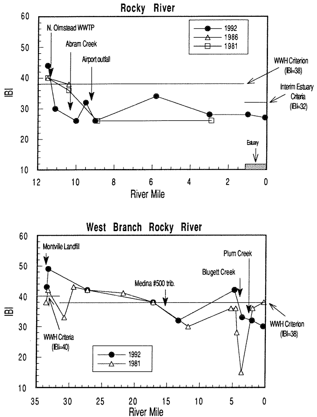
Figure 36. Longitudinal trends of the Index of Biotic Integrity (IBI) in the Rocky River mainstem and the West Branch Rocky River study areas; 1981,1986 and 1992.
