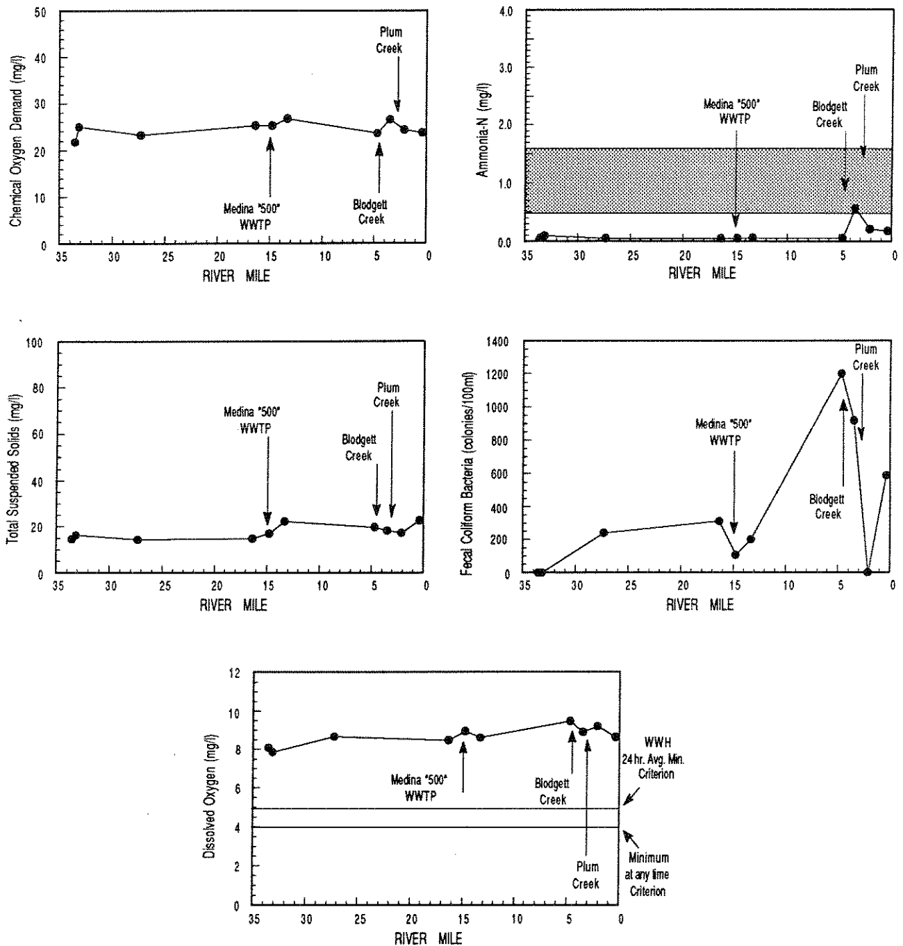
Figure 18. Longitudinal trend of mean chemical oxygen demand, ammonia-N, total suspended solids, fecal coliform bacteria, and dissolved oxygen in the West Branch Rocky River study area, 1992. Shaded area represents the ammonia-N criteria range between the 90th and 25th percentile pH and temperatures.
