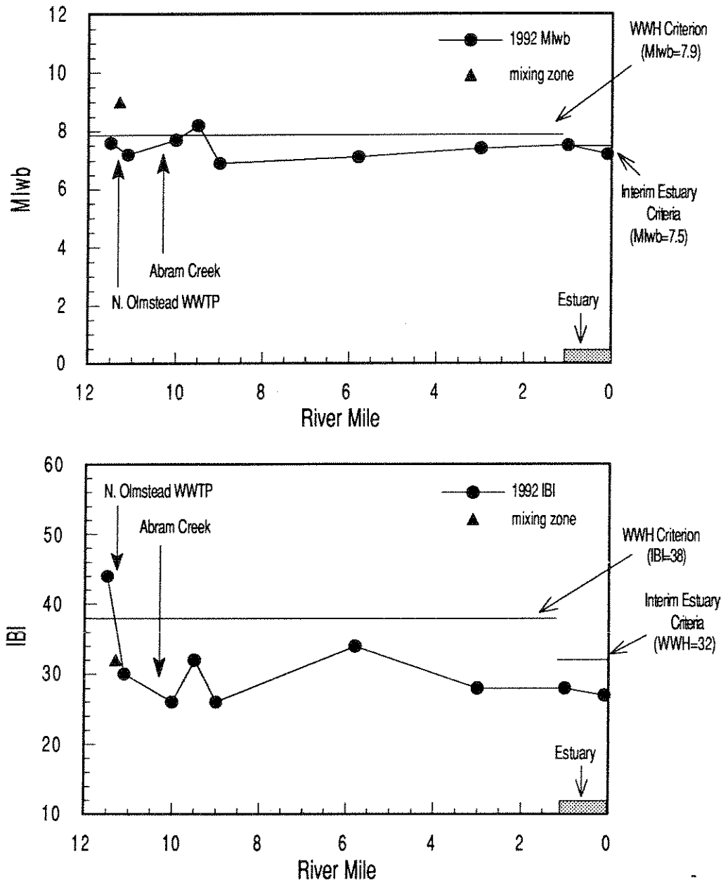
Figure 8. Longitudinal trend of the Index of Biotic Integrity (IBI; lower) and the Modified Index of Well-Being (MIwb; upper) in the Rocky River, 1992.
