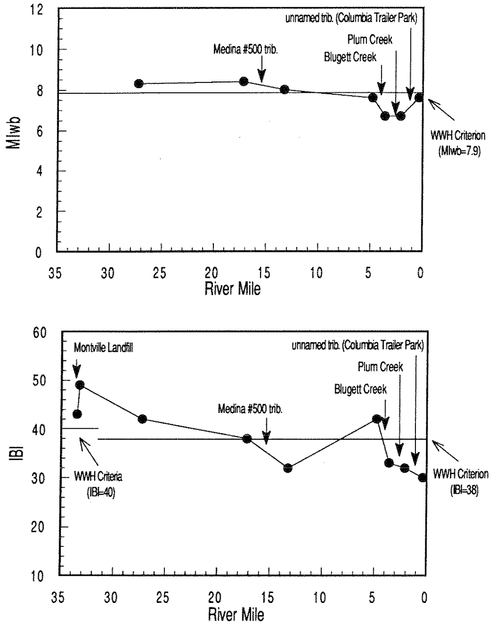
Figure 20. Longitudinal trend of the Modified Index of Well-Being (MIwb; upper) and the Index of Biotic Integrity (IBI; lower) in the West Branch Rocky River, 1992.
