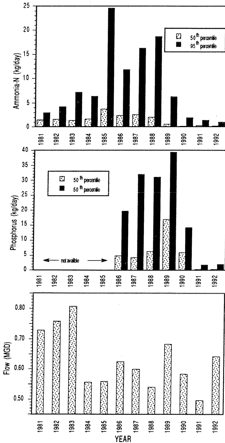
Figure 21. Average flow (MGD) and annual loadings (kg/day) of ammonia-N, phosphorus and from the North Royalton "B" WWTP to Baldwin Creek, 1981-1992.
