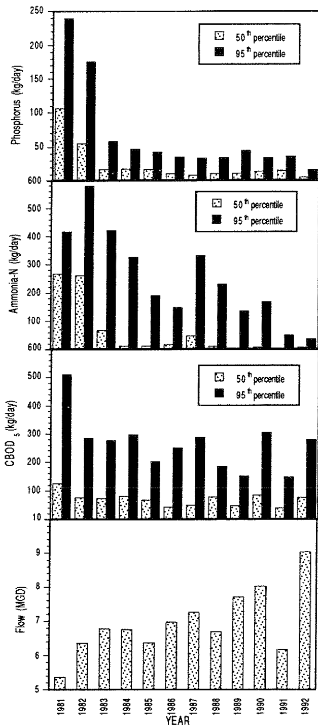
Figure 17. Average flow (MGD) and annual loadings (kg/day) of phosphorus, ammonia-N, and CBOD 5 from the Medina 500 WWTP to the West Branch Rocky River, 1981-1992. CBOD 5 loadings for 1981-1984 are calculated based on reported biochemical oxygen demand (BOD 5 ) values.
